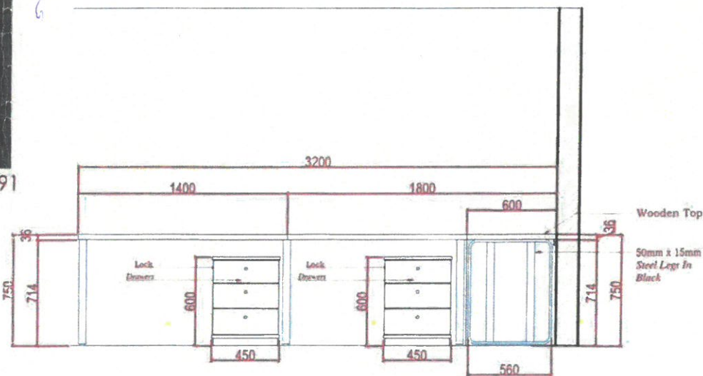
FRONT ELEVATIONS
