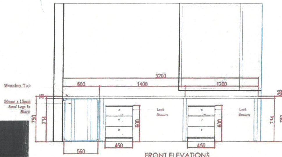
FRONT ELEVATIONS
